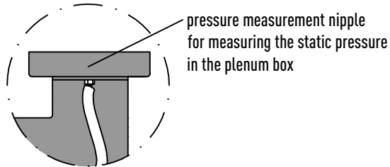
detail "X", scale 1:5
