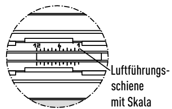
Detail "Z", M 1:5
